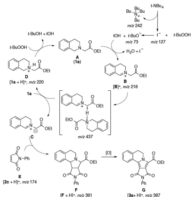
Scheme 1 Proposed mechanism.
