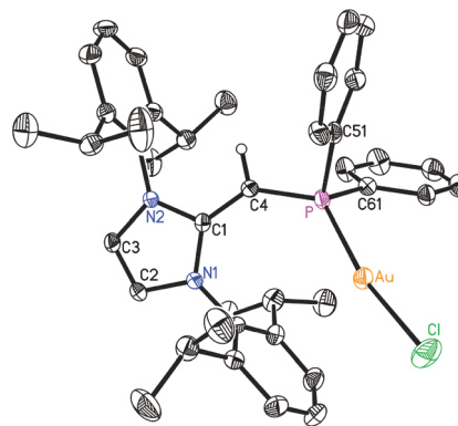
Fig. 8 Molecular structure of 9 with thermal ellipsoids at the 30% probability level. The hydrogen atom attached to C(4) is shown with an arbitrarily small thermal parameter; all other hydrogens have been omitted for clarity. Selected bond lengths (Å) and angles (°): Au–P 2.2334(8), Au–Cl 2.2914(10), P–C(4) 1.741(3), C(1)–C(4) 1.381(4), P–C(51) 1.831(3), P–C(61) 1.826(3); P–Au–Cl 168.72(4), C(4)–P–Au 128.48(11), P–C(4)–C(1) 136.9(3), C(4)–P–C(51) 99.84(15), C(4)–P–C(61) 109.43(15), Au–P–C(51) 106.45(11), Au–P–C(61) 106.46(11).
