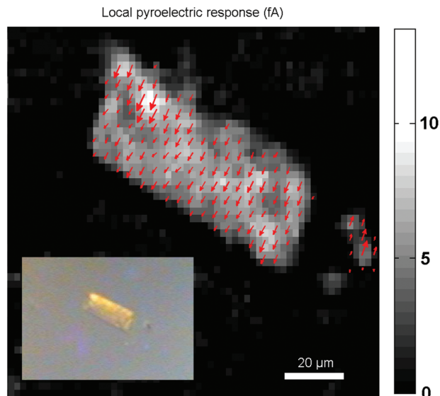
Fig. 7 The local pyroelectric response map reveals a unipolar response from the \text{Fe}(\text{OH}/\text{F})(\text{BDC}) \cdot [\text{H}_2\text{O}] crystal. Modulation frequency is 2025 Hz, laser power is 100 mW. Inset: optical image.
