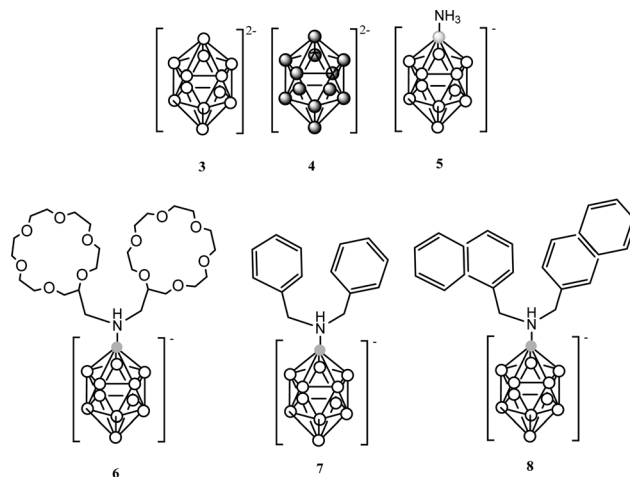
Chart 3 Chemical structures of the [B 12 H 12 ] 2− (3) and its derivatives (4)–(8). White circles correspond to B–H while the dark circles to B–Li vertices and the grey circles to a B atom.
