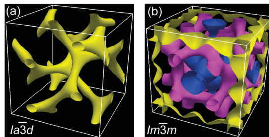
Fig. 4 Reconstructed EDMs: (a) of a unit cell of the Cub// Ia\bar{3}d phase of AB8 only showing the high density regions and (b) of the Im\bar{3}m approximate of the Cub/ I432 phase of AB14 showing the three distinct iso-surfaces with different colour.
