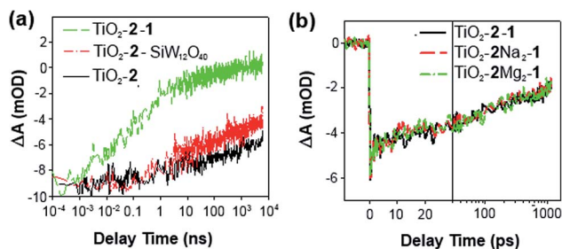
Fig. 5 (a) Ground state bleach recovery kinetics of \text{TiO}_2 - 2 (black), \text{TiO}_2 - 2 - \text{SiW}_{12}\text{O}_{40} (red) and \text{TiO}_2 - 2 - 1 . (b) Ground state bleach recovery kinetics of \text{TiO}_2 - 2 - 1 (black), \text{TiO}_2 - 2 - \text{Na}_2 - 1 (red) and \text{TiO}_2 - 2 - \text{Mg}_2 - 1 (green).
