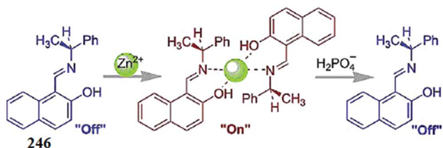
Fig. 210 Chemical structure of receptor 246, proposed ligand–zinc complexation mechanism and reversibility.
