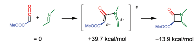
Scheme 8 DFT computed (DFT-D3, BP86, def2-TZVP) uncatalysed coupling of the free (uncoordinated) ketene and imine substrates.
