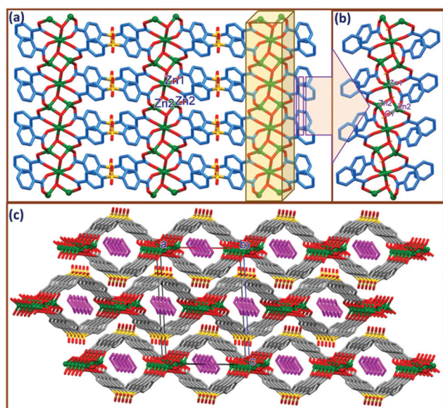
Fig. 2 (a) Two dimensional coordination polymeric network of {[Zn 3 (μ-OH) 2 (SDB) 2 ](PPZ)} n in 2, (b) close-up view depicting the coordination environment in 2, (c) packing diagram depicting the staggering of adjacent 2D sheets and through cylindrical channels down the b -axis with the encapsulated piperazine molecule.
