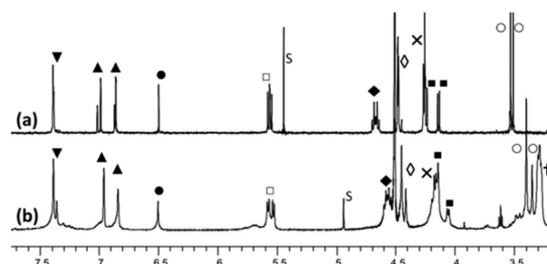
Fig. 1 1 H NMR spectra (500 MHz, 300 K) of (a) organosoluble Rim 3 ligand in CD 3 CN and (b) water-soluble WRim 3 ligand in D 2 O (2.6 mmol). (▼) HAR. “down”; (▲) HIm; (●) HAR. “up”; (□) and (■) OCH 2 O; (◆) –CHAR; (◇) CH 2 Im; (X) ArCH 2 O; (○) NCH 3 ; (♣) –CHAR; (†) CH 2 N + Me 3 . S stands for solvent.
