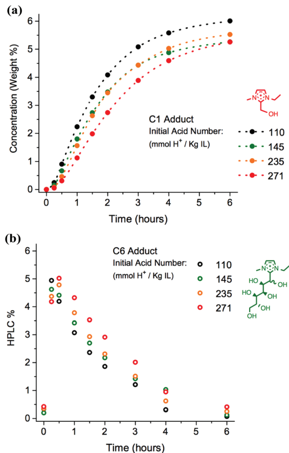
Fig. 11 Comparison of adduct formation for [\text{C}_2\text{C}_1\text{im}][\text{OAc}] , 1a + 10 wt% D-(+)-glucose, 12 , with differing initial acid numbers (110–271 mmol \text{H}^+ \text{kg}^{-1} IL), heated at 120 °C for 24 hours: (a) wt% of the C1 adduct, [\text{C}_2\text{C}_1(\text{HO})\text{C}_1^2\text{im}]^+ ; (b) HPLC% of the intermediate C6 adduct. Graphs are shown in the range t_0 – t_6 , for clarity.
