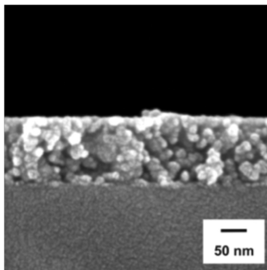
Fig. 20 Cross-sectional SEM image of \text{MgF}_2 thin film annealed at 500^\circ\text{C} . Reproduced from ref. 33 with permission of The Royal Society of Chemistry.
