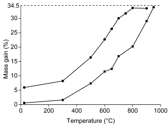
Fig. 3 Mass gain (%) of the <400\ \mu\text{m} (■) and <80\ \mu\text{m} (●) NdFeB magnet powder as a function of the temperature at which it was held for 1 h. The dashed line is drawn at 34.5%, which is the maximum mass gain determined with TGA.
