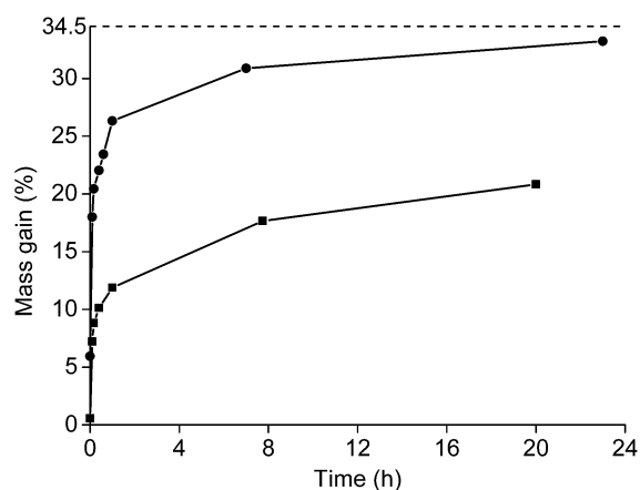
Fig. 4 Mass gain (%) of the <400\ \mu\text{m} (■) and <80\ \mu\text{m} (●) NdFeB magnet powder as a function of the roasting time at a temperature of 650\ ^\circ\text{C} . The dashed line is drawn at 34.5%, which is the maximum mass gain determined with TGA.
