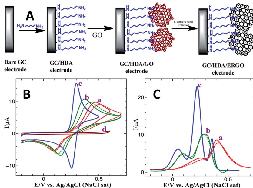
Fig. 8 (A) Schematic illustration for the fabrication of ERGO modified GCE, (B) CVs obtained for the oxidation of 0.5 mM of DA at (a) bare GC, (b) GC/HDA/GO, and (c) GC/HDA/ERGO electrodes in 0.2 M PB solution (pH 5.5) at a scan rate of 50\ \text{mV s}^{-1} . Solid line: first cycle; dotted line: eighth cycle. (C) DPVs obtained for the oxidations of each 0.5 mM of AA, DA, and UA at (a) bare GCE, (b) GC/HDA/GO, and (c) GC/HDA/ERGO electrodes in 0.2 M PB solution. Solid line: first cycle; dotted line: eighth cycle. Reprinted with permission from ref. 79, Copyrights (2013) American Chemical Society.
