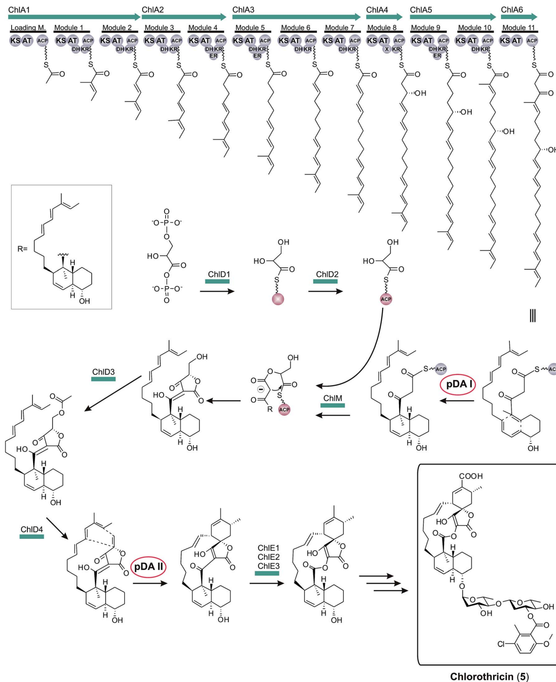
Fig. 9 Model for chlorothricin ( 5 ) biosynthesis. The polyketide synthase multi-enzyme complex (ChIA1-6) synthesizes the linear chlorothricin precursor and a first Diels–Alder reaction (pDA = postulated Diels–Alder reaction I, pDA I) is postulated to yield the trans -decalin unit. This molecule is then fused to the preactivated and ACP-coupled C 3 -unit, derived from 1,3-bisphosphoglycerate. Tetronic acid formation and maturation steps depicted in this figure are postulated by the authors of this review based on observations made for the biosynthesis of agglomerin A (ChID1-4 and ChIM: protein set encoded by the conserved “glycerate utilization operon”). A second formal Diels–Alder reaction (pDA II) is proposed to take place between the exocyclic methylene group of the tetronic acid moiety and a pair of conjugated double bonds in the tail region of the linear polyketide, thereby generating a premature macrocycle. Three candidate enzymes (ChIE1-3) were suggested to catalyze the Baeyer–Villiger oxidation reaction which introduces an oxygen atom into the macrocycle. Further decoration of the macrolactone ring, mainly glycodiversification reactions, yields the final chlorothricin structure ( 5 ).
