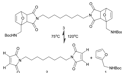
Scheme 2 DA and rDA reactions in compound 3 .
