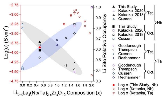
Fig. 9. Relationship between composition, \text{Log}(\sigma) at room temperature, 12,26 and tetragonal (Tet.) and octahedral (Oct.) Li site occupancy 16,22,24,25,27,28 for Nb-substituted \text{Li}_{5+x}\text{La}_3\text{Nb}_{2-x}\text{Zr}_x\text{O}_{12} (LLNZO) and Ta-substituted \text{Li}_{5+x}\text{La}_3\text{Ta}_{2-x}\text{Zr}_x\text{O}_{12} (LLTZO) compositions from x = 0 to x = 2 . Trend in cubic LLNZO and LLTZO octahedral site occupancy increasing with Li content illustrated with blue ellipse and tetragonal site occupancy decreasing with increasing Li content illustrated with grey ellipse. The \text{Log}(\sigma) at room temperature for LLNZO and LLTZO compositions are highlighted in red.
