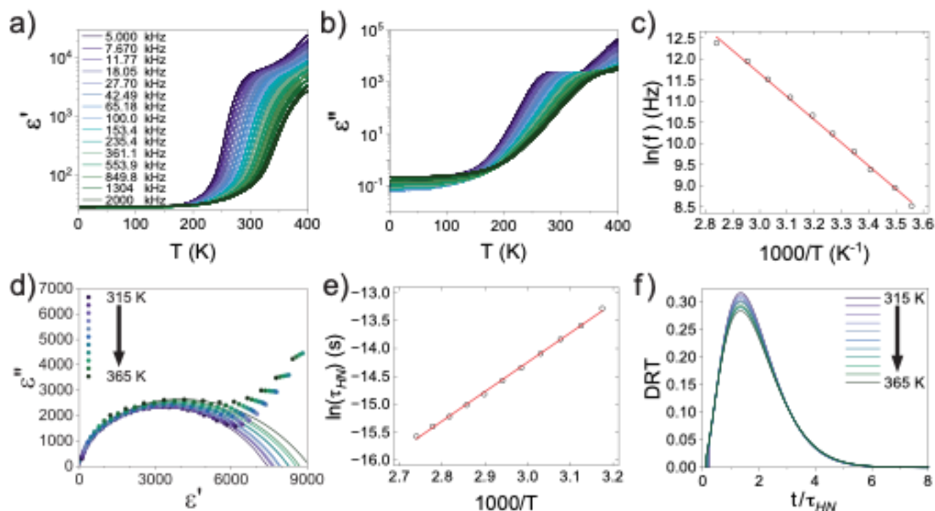
Fig. 8 (a) Dielectric constant ( \epsilon' ) and (b) dissipation ( \epsilon'' ) of single crystal Li 5.5 -LLNZO as a function of temperature at frequencies from 5–2,000 kHz. (c) Arrhenius fitting of frequency vs. temperature ( R^2=0.997 ). Data shown as black circles, linear fit in red. (d) Cole–Cole plots of the complex dielectric constant from 315–365 K in 5 K increments (symbols) and Havriliak–Negami function fittings (lines). (e) Arrhenius fitting of Havriliak–Negami relaxation time \tau_{HN} vs. temperature from 315–365 K ( R^2=0.998 ). Data shown as black circles, linear fit in red. (f) Distribution of relaxation time (DRT) as a function of time normalized to Havriliak–Negami relaxation time \tau_{HN} from 315–365 K in 5 K increments.
