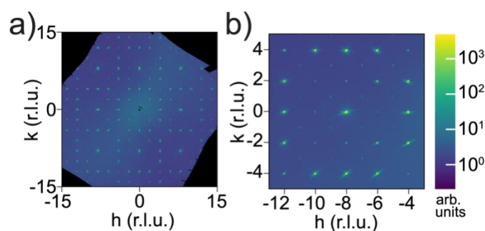
Fig. 6 (a) Synchrotron single crystal scattering pattern for Li 5.5 -LLNZO in the hk0 plane. (b) Enlarged region of hk0 scattering plane showing additional Bragg reflections in hk0 with h+k = 2n and in h00 or 0k0 with h or k = 4n+2 .
