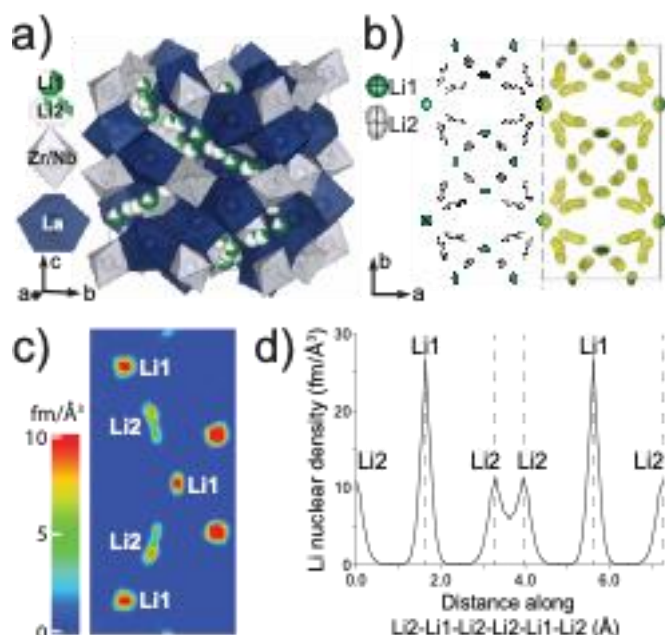
Fig. 5 (a) Unit cell structure for Li 5.5 -LLNZO determined from neutron single-crystal diffraction. (b) Left: Anisotropic thermal displacements of Li sites. Right: Nuclear density iso-surfaces (0.399 fm/Å 3 ) based on MEM analysis overlaid on displacement ellipsoids. (c) 2D nuclear density map from MEM analysis through Li 1 -Li 1 -Li 1 direction. (d) MEM-determined Li nuclear density along Li 2 -Li 1 -Li 2 -Li 2 -Li 1 -Li 2 direction.
