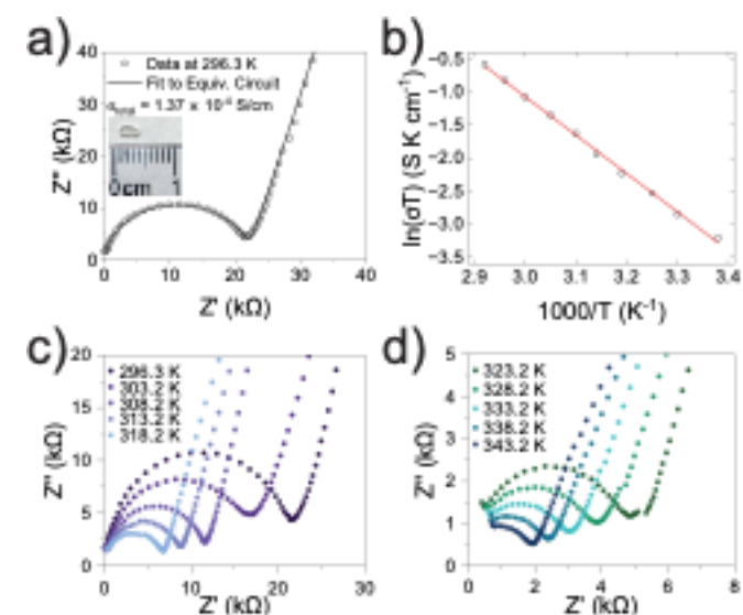
Fig. 7 (a) Nyquist plot of Li 5.5 La 3 Nb 1.5 Zr 0.5 O 12 single-crystal sample from EIS in argon atmosphere at 296.3 K. Inset: polished crystal plate for EIS measurements. (b) Arrhenius relationship and line of best fit for \ln(\sigma T) vs 1000/T impedance data from 296.3 to 343.2 K ( R^2=0.998 ). Data shown as black circles, linear fit in red. (c, d) EIS spectra at progressive temperature points from 296.3 to 343.2 K.
