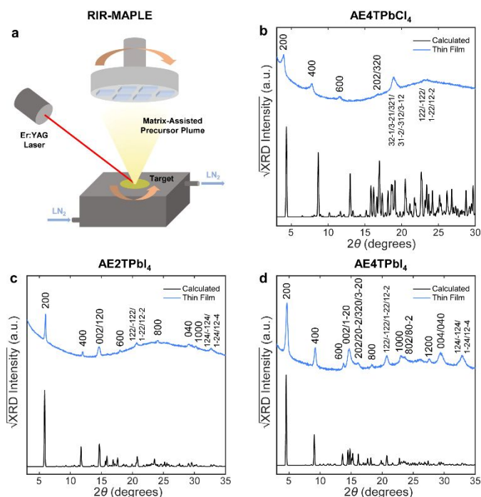
Figure 2. Schematic of the RIR-MAPLE process (a), and Cu K\alpha XRD patterns of oligothiophene perovskite films deposited by RIR-MAPLE, referenced against patterns calculated using computationally optimized structures from van der Waals corrected semilocal DFT: (b) \text{AE4TPbCl}_4 , (c) \text{AE2TPbI}_4 , and (d) \text{AE4TPbI}_4 . Comparison of the film XRD patterns against the calculated patterns indicates that all of the peaks in the former may be assigned to Miller indices corresponding to reasonably prominent peaks in the latter. Similar sets of reflections (e.g., h00 , 0k0 , 122 ) appear in the patterns of both ( \text{AE2T/AE4T} ) \text{PbI}_4 , indicating similar texture in these closely related materials. The \text{AE4TPbCl}_4 pattern contains fewer and less-well-defined peaks. However, features resembling those in the other patterns are evident, such as the first three h00 reflections, which decrease in intensity in a manner consistent with the predicted pattern and the other two perovskites. The theory-derived \text{AE4TPbCl}_4 pattern slightly underestimates the lattice constant along the a axis; however, the inferred values are still broadly consistent with the expected structure. Note that another recent computational study on \text{AE4TPbCl}_4 predicts a similar value for the interlayer lattice parameter as our DFT calculations; 2 however, also note that relatively subtle changes in the configuration of the quaterthiophene cations can have substantial impact on the lattice parameters in the DFT-predicted structures, as explored further in the Supporting Information (Figure S2, Table S2). Accurate determination of all subtleties of the structure would require the growth and XRD refinement of single crystals, which is beyond the scope of this work. Importantly, the key optoelectronic properties reported below are experimentally derived and thus not affected by small structural deviations between the computationally assumed model and the experimental material.
