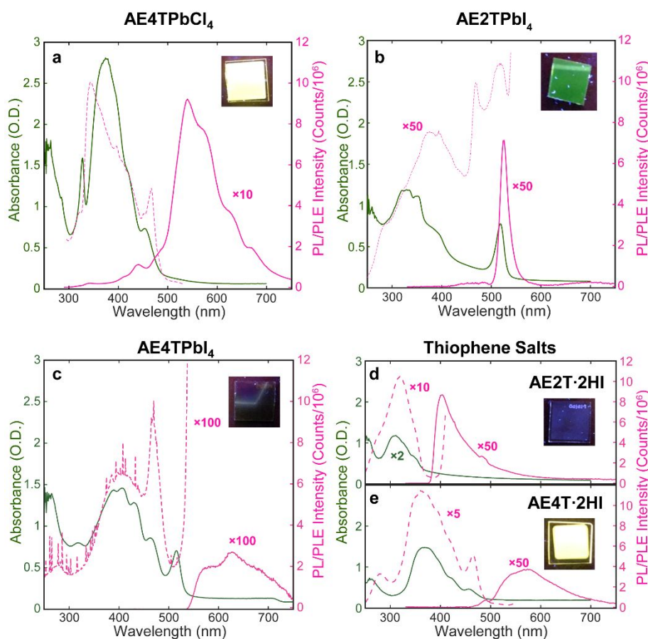
Figure 3. UV-vis (solid green lines), PL (solid pink lines) and PLE (dashed pink lines) spectra of oligothiophene COP and precursor salt thin films deposited by RIR-MAPLE: (a) AE4TPbCl 4 , (b) AE2TPbI 4 , (c) AE4TPbI 4 , (d) AE2T·2HI and (e) AE4T·2HI. PL spectra are collected using excitation by a monochromated Xe lamp at 280 nm (a) or 335 nm (b-e), at energies high enough to generate excitons in both parts of the perovskite structure. PLE spectra are collected using a monochromated Xe lamp at emission wavelengths of 600 nm (a,e), 560 nm (b), 570 nm (c) or 430 nm (d)—i.e., near the maximum intensity of the PL spectrum. In (b-d), the increase in the PLE signal at longer wavelengths is due to collection of scattered excitation light. All optical data are scaled as noted in the figure in order to be plotted on the same axes. Insets: photographs of perovskite and thiophene salt films under a 365 nm UV lamp, displaying the characteristic luminescence of each composition (or lack thereof, in the case of AE4TPbI 4 ).
