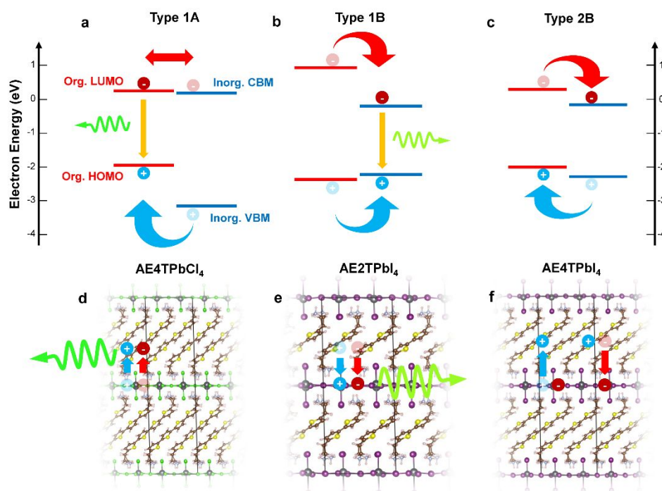
Figure 1. Schematics of hybrid spin-orbit coupled DFT predicted internal band/molecular orbital alignments (a–c) and anticipated exciton/luminescence behavior (d–f) in AE4TPbCl 4 (a,d), AE2TPbI 4 (b,e) and AE4TPbI 4 (c,f). AE4TPbCl 4 is expected to exhibit a Type 1A quantum well structure, wherein excitons generated in the inorganic part migrate to the organic part, leading to luminescence characteristic of the quaterthiophene. AE2TPbI 4 is predicted to exhibit Type 1B behavior, wherein excitons generated in the organic part migrate to the inorganic part, leading to luminescence from the lead halide sheet. AE4TPbI 4 is expected to exhibit Type 2B behavior, where excitons generated in either part dissociate across the organic-inorganic interface, inhibiting radiative recombination and quenching luminescence. Band positions are drawn to scale based on the calculations of Liu et al. 3 for AE4TPbI 4 and AE4TPbCl 4 , and on the calculations for AE2TPbI 4 reported in this work. Note that, within the accuracy limits of currently applicable first-principles calculations, the organic LUMO of AE4TPbCl 4 is essentially indistinguishable from the inorganic VBM; prior experimental results, 16, 17 as well as those described in this work, support its assignment as a Type 1A structure.
