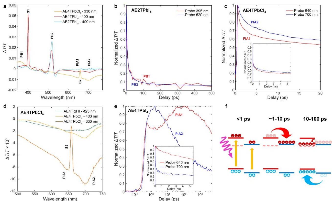
Figure 4. Transient absorption spectra of the AE4TPbI 4 , AE2TPbI 4 , and AE4TPbCl 4 samples after a pump-probe delay time of 15 ps (a); decay kinetics of selected features in AE2TPbI 4 (b), AE4TPbCl 4 (c,d), and AE4TPbI 4 (e); schematic of carrier transfer in AE4TPbI 4 (f), wherein the triplet state is represented by the dashed line and the band positions are the same as in Figure 1. The features labeled S1 and S2 in (a) and (d) correspond to scattered light from the pump beam at 400 nm and 660 nm, respectively.
