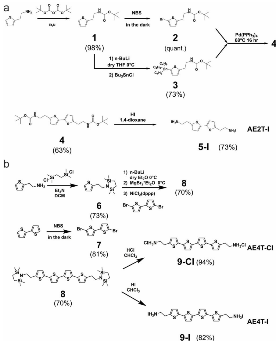
Scheme 1. Synthesis pathways for (a) bi- and (b) quaterthiophene halide salts used in this study. Detailed discussion of the synthesis of each compound shown in the Scheme is given in the Methods section and ESI. Briefly, AE2T-2HI is synthesized starting from a thiophene-2-ethylamine precursor via a method reported by Harvey and Tovar. 1 The amine is first protected using a tert-butyloxycarbonyl group to form tert-butyl (2-(thiophen-2-yl)ethyl)carbamate ( 1 ). The bithiophene diamine building blocks are prepared by treating 1 with N-bromosuccinimide (NBS) to form tert-butyl (2-(5-bromothiophen-2-yl)ethyl)carbamate ( 2 ) or tributyl tin chloride to form tert-butyl (2-(5-(tributylstannyl)thiophen-2-yl)ethyl)carbamate ( 3 ). 2 and 3 are then coupled via Stille reaction to form di-tert-butyl ((2,2'-bithiophene)-5,5'-diylbis(ethane-2,1-diyl))dicarbamate ( 4 ), which is thereafter deprotected using hydriodic acid, yielding the desired AE2T-HI product ( 5-I ). AE4T-2HX salts are synthesized starting from bithiophene and thiophene-2-ethylamine precursors via a method reported by Muguruma et al. 4 The amine is protected to form 2,2,5,5-tetramethyl-1-(2-(thiophen-2-yl)ethyl)-1,2,5-azadisilolidine ( 6 ), while bithiophene is brominated with NBS to form 5,5'-dibromo-2,2'-bithiophene ( 7 ). 7 and lithiated 6 are thereafter linked via Kumada coupling reaction to yield the protected quaterthiophene diamine 5,5'''-bis(2-(2,2,5,5-tetramethyl-1,2,5-azadisilolidin-1-yl)ethyl)-2,2':5',2'':5'',2''':5'''-quaterthiophene ( 8 ), which is thereafter deprotected using the appropriate hydrohalic acids, yielding the desired ammonium salts AE4T-2HCl ( 9-Cl ) and AE4T-2HI ( 9-I ).
