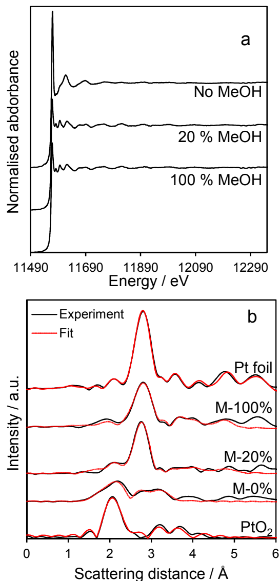
Fig. 6. Transmission Pt L_{III} -edge (a) normalized XANES spectra and (b) radial distribution functions of Pt/TiO 2 catalysts. Pt foil and oxide references shown for comparison.
