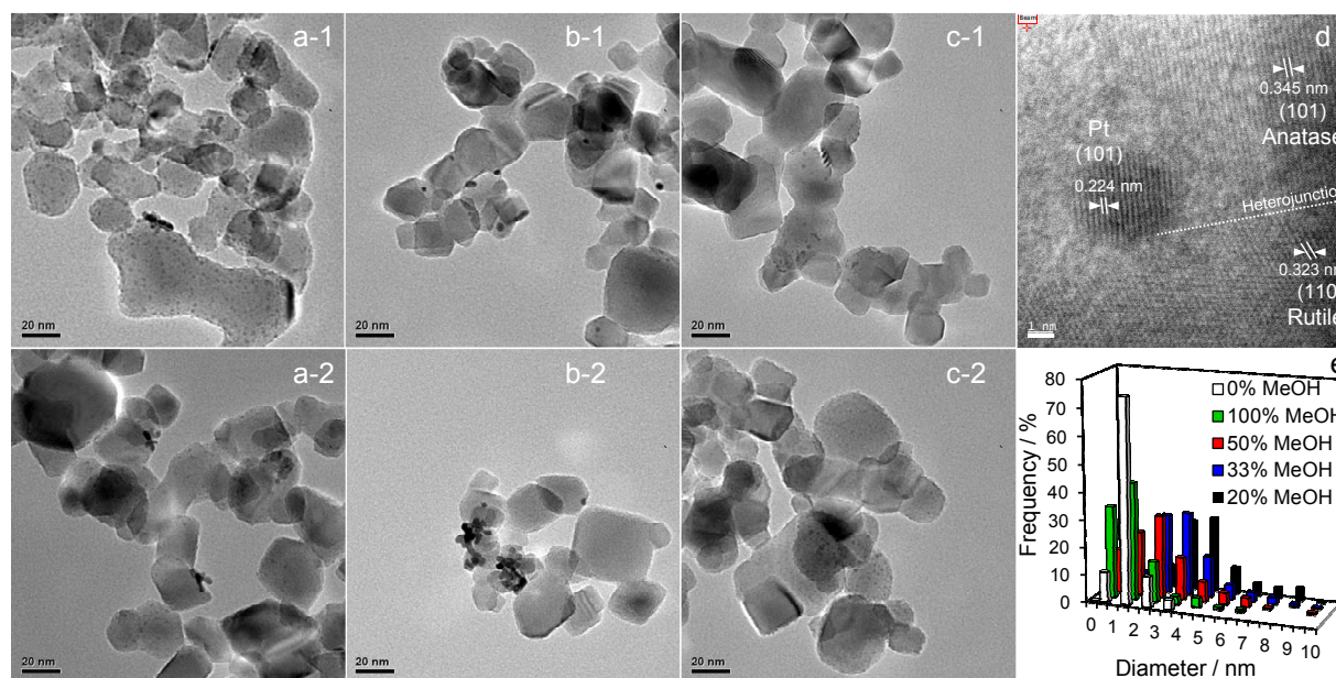
Fig. 3. Representative bright-field HRTEM images of (a1-2) 100%, (b1-2) 20%, and (c1-2) 0% MeOH 1 wt% Pt/TiO 2 , (d) an individual Pt metal nanoparticle at the interface between anatase and rutile crystallites, and (e) particle size distributions as a function of methanol concentration during PD.
