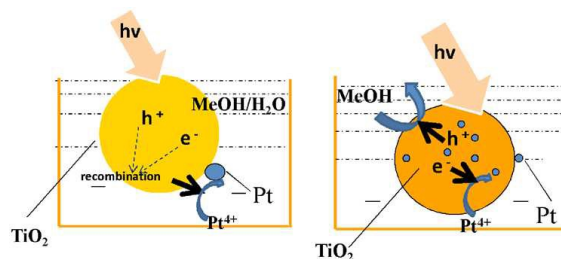
Fig. 7. Schematic of the proposed mechanism for methanol-promoted PD of highly dispersed platinum nanoparticles over titania.
