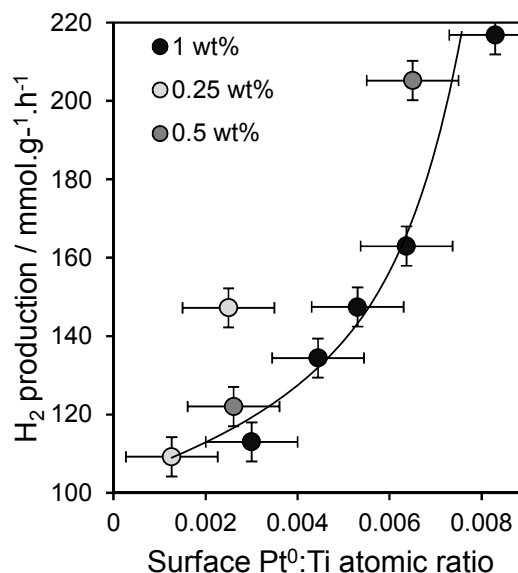
Fig. 10. Relationship between the rate of photocatalytic hydrogen production and dispersion of metallic Pt metal for Pt/ \text{TiO}_2 catalysts prepared via PD.
