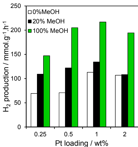
Fig. 9. Photocatalytic hydrogen evolution over Pt/ \text{TiO}_2 catalysts as a function of Pt loading and methanol concentration during PD.
