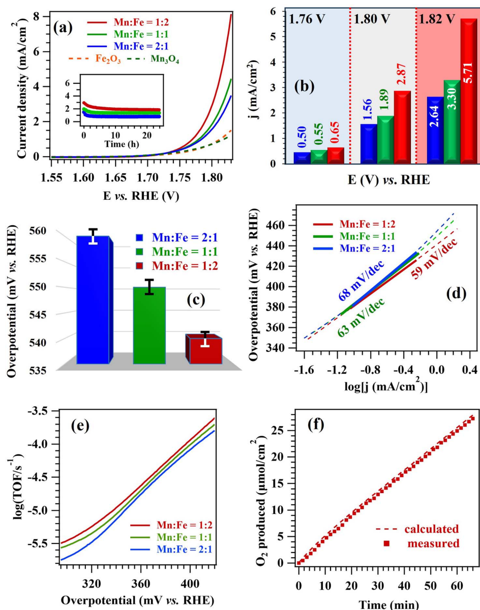
Fig. 10 Electrochemical OER performances of MFO systems in simulated alkaline seawater. (a) iR -corrected LSV traces. Mn 3 O 4 and Fe 2 O 3 curves are also reported for comparison. Inset: chronoamperometric tests for MFO electrocatalysts, performed at 1.80 V vs. RHE. (b) Current densities at different bias values. (c) Overpotentials at 1 mA cm -2 . (d) Tafel plots; dashed and continuous lines correspond to experimental and fitting curves, respectively. (e) TOF curves vs. overpotential for the target electrocatalysts. (f) O 2 evolution vs. time for the Mn : Fe = 1 : 2 specimen. The dashed curve was calculated assuming a 100% Faradaic efficiency.
