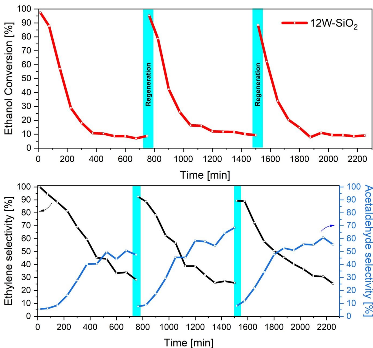
Figure 14. Regeneration of 12W-SiO 2 catalyst and ethanol conversions and product selectivity at 420 °C with WHSV 7.09 h -1 .
