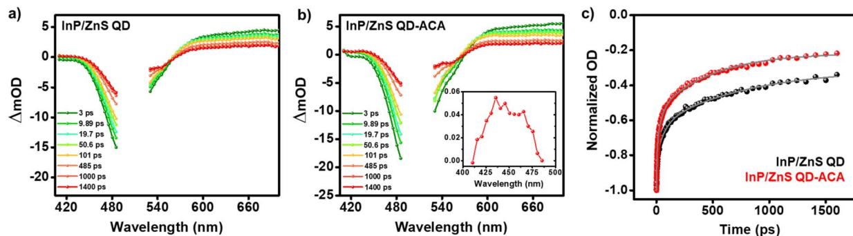
Fig. 2 fs-TA spectra at indicated time delays upon 500 nm excitation of (a) InP/ZnS QDs and (b) InP/ZnS QD-ACA. Inset of (b) shows the absorption feature of {}^3\text{ACA}^* at \sim 430 nm obtained by subtracting the normalized spectra corresponding to 1400 ps and 3 ps time delays. (c) Kinetics of the GSB bleach recovery of InP/ZnS QDs with and without ACA ligands.
