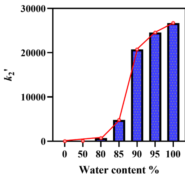
Fig. 4 Graphical representation of relative second-order rate constant values ( k_2' ) for the reaction of 2 (0.05 mM) with BNAH at 293 K at different water ratios where k_2' = k_2 \cdot \text{H}_2\text{O}/k_2 \cdot \text{CH}_3\text{CN} .
