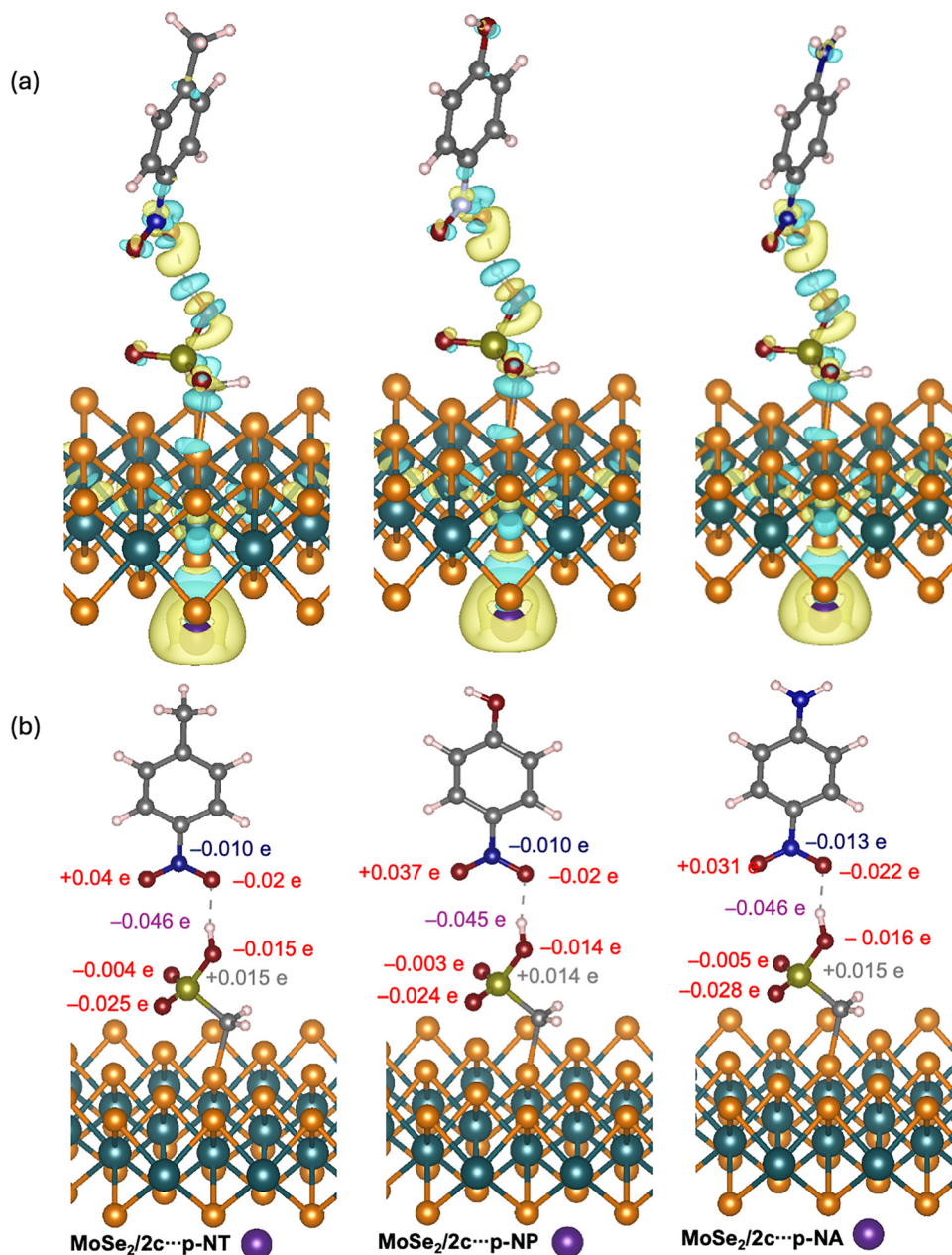
Fig. 4 (a) Electronic density differences and (b) Löwdin partial charges for \text{MoSe}_2/2\text{c} interacting with p -NT, p -NP, and p -NA target molecules. The charge density differences were plotted at a density isovalue of 2.5 \times 10^{-3} e \text{ Bohr}^{-3} .
