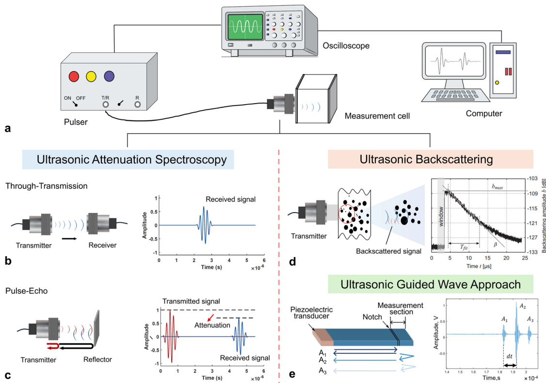
Fig. 8 Experimental ultrasonic measurement configurations. (a) Electronical devices in a typical experimental setup; (b) the ultrasonic attenuation spectroscopy with transducer arranged in through-transmission and (c) pulse-echo manners; (d) ultrasonic backscattering measurement. The left plot shows the typical setup and the right plot (reproduced from ref. 175 with permission) a typical backscattered signal time trace; (e) ultrasonic guided wave approach for macroscopic property measurement. The left plot shows a dip-stick setup and the right the typical time trace to evaluate viscosity-induced attenuation (reproduced from ref. 177 licensed under CC BY-NC 4.0).
