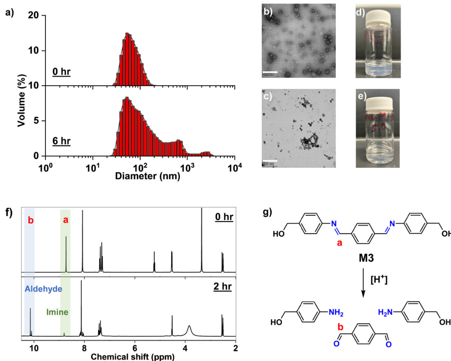
Fig. 5 DLS diagrams of aqueous P-Im3-Aq nanogels incubated at pH 5.0 over 6 h (a); their TEM images (scale bar = 500 nm) (b and c), and digital images (d and e); and overlaid 1 H NMR spectra of M3 in DMSO- d 6 /HCl (f) and acid-catalyzed hydrolysis of benzoic imine bond in M3 (g).
