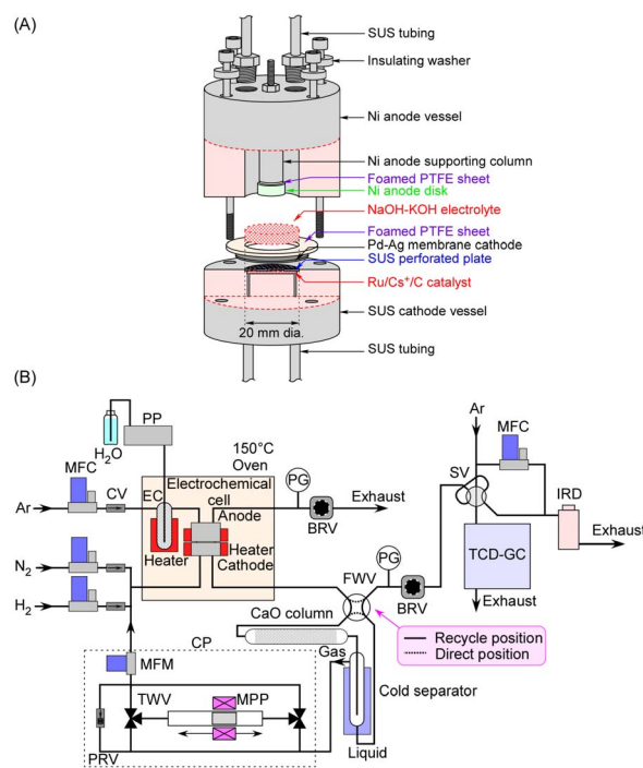
Fig. 2 Detailed cross-sectional view of the electrochemical cell (A) and diagram of the gas lines (B). PP: plunger pump, MFC: mass flow controller, CV: check valve, EC: evaporation chamber, PG: pressure gauge, BRV: back-pressure regulating valve, FWV: four-way valve, CP: circulation pump, MFM: mass flow meter, PRV: pressure relief valve, TWV: electric three-way valve, MPP: magnetic piston pump, SV: sampling valve, TCD-GC: gas chromatograph with a thermal-conductivity detector, and IRD: infrared absorption \text{NH}_3 detector.
