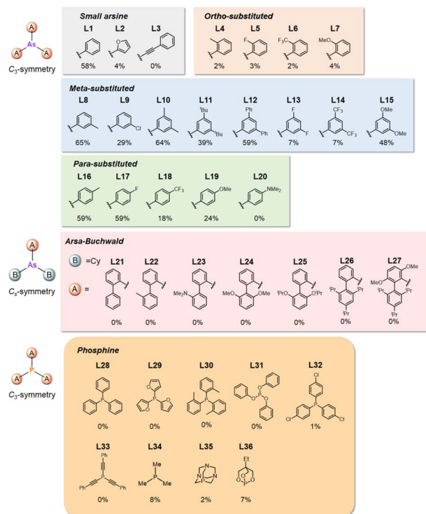
Fig. 2 o -, m -, and p -substituted C_{3v} - and C_{3h} -type arsine and phosphine ligands. The NMR yield of the difunctionalized product 1 (Scheme 1) is shown below each structure.
