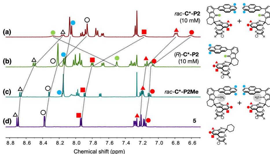
Fig. 2 Partial 1 H NMR spectra of (a) rac -C*-P2 (10 mM), (b) ( R )-C*-P2 (10 mM), (c) rac -C*-P2Me (6.1 mM), and (d) 5 (23 mM) in CDCl 3 at T = 298 K. Proton resonances are labeled with the symbols denoted in the chemical structures.
