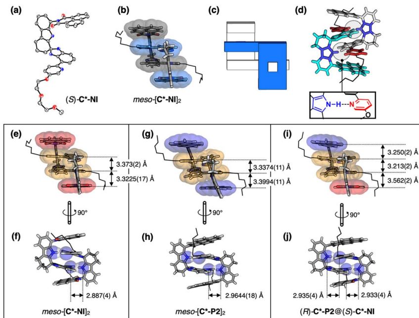
Fig. 1 X-ray structure of C*-NI as (a) ORTEP diagram with thermal ellipsoids at the 50% probability level, (b) capped-stick representation built with crystallographically determined atomic coordinates of meso -[C*-NI] 2 , and (c) brick-like schematic representation. (d) Intermolecular N indole -H...N pyridyl hydrogen bond of meso -[C*-NI] 2 . (e and f) meso -[C*-NI] 2 , (g and h) meso -[C*-P2] 2 , and (i and j) quasi-racemate ( R )-C*-P2@( S )-C*-NI with metric parameters for \pi - \pi stacking and hydrogen bonding.
