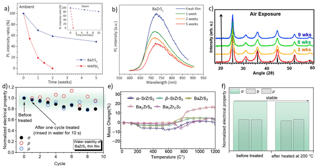
Fig. 19 Stability of \text{BaZrS}_3 against extrinsic factors. (a) Plot comparing the PL intensity of \text{BaZrS}_3 and \text{MAPbI}_3 films under ambient conditions over time, with an inset showing the variation in PL intensity upon exposure to steam. (b) Plot depicting the PL intensity of \text{BaZrS}_3 over several weeks of exposure to ambient conditions. (a) and (b) Reproduced with permission. 62 Copyright 2020, Wiley. (c) Plot illustrating the structural stability of \text{BaZrS}_3 nanoparticles over several weeks in air. (c) Reproduced with permission. 136 Copyright 2022, Royal Society of Chemistry. (d) Plot demonstrating the superior water stability of \text{BaZrS}_3 film by assessing carrier properties after water rinsing. (d) Reproduced with permission. 48 Copyright 2023, Elsevier. (e) Plot showing the exceptional thermal stability of \text{BaZrS}_3 powder up to 500 °C. (e) Reproduced with permission. 64 Copyright 2018, Springer Nature. (f) Plot indicating minimal changes in the carrier properties of \text{BaZrS}_3 after heat treatment at 200 °C. (f) Reproduced with permission. 48 Copyright 2023, Elsevier.
