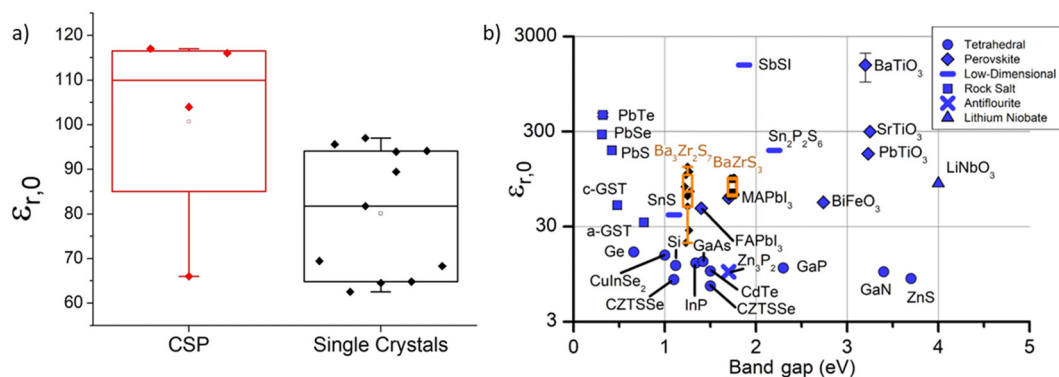
Fig. 4 Dielectric constant of \text{BaZrS}_3 and other inorganic materials. (a) Comparison of the dielectric constant for densified \text{BaZrS}_3 obtained through cold-sintering and single crystal \text{BaZrS}_3 . (b) Plot illustrating the relationship between the dielectric constant and bandgap for various inorganic materials. (a) and (b) Reproduced with permission. 69 Copyright 2021, Springer Nature.
