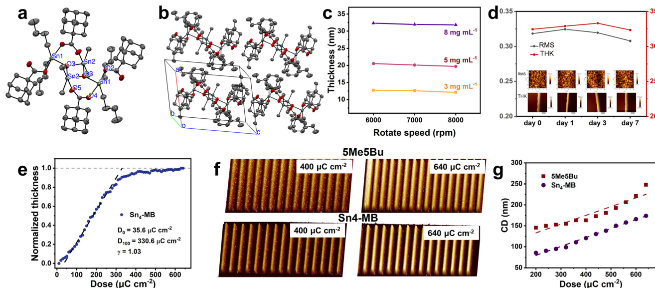
Fig. 1 (a) and (b) Single crystal structures of Sn4-MB. The hydrogen atoms were omitted for clarity; (c) thickness of films obtained from different concentrations of Sn4-MB precursor solutions at different rotational speeds; (d) time-dependent variation in surface roughness (RMS) and film thickness (THK) of Sn4-MB films at days 0, 1, 3, and 7 after spin-coating. Insets show AFM surface topography (top row) and cross-sectional profiles (bottom row), corresponding to the same time points from left to right; (e) contrast curves of Sn4-MB; (f) AFM images of L/3S dense line patterns (100 nm pitch) generated from Sn4-MB and 5Me5Bu resists under area-exposure at electron beam doses of 400 and 640 μC cm -2 ; (g) periodic line CD of Sn4-MB and 5Me5Bu films under area-exposure as a function of exposure dose.
