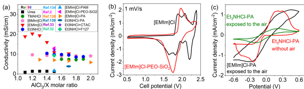
Fig. 15 (a) Ionic conductivity of various AlCl 3 /X electrolytes. X = [EMIm]Cl (10–20 mS cm -1 ), TMAHCl (average ~7.5 mS cm -1 ), Et 3 NHCl (~9.6 mS cm -1 ), [BMIm]Cl (~9.4 mS cm -1 ), and urea (~1.3 mS cm -1 ) were measured at 25 °C. 98 [EMIm]Cl-PAM (1.66 × 10 -3 S cm -1 , measured at 20 °C) is gel polymer electrolyte made from PEO, AlCl 3 /[EMIm]Cl (1.5 : 1) and an additive-fumed SiO 2 . 2 [EMIm]Cl-PA (5.89 to 7.24 mS cm -1 , measured at room temperature) and Et 3 NHCl-PA (3.86 mS cm -1 , measured at 25 °C) is PA-based gel polymer electrolyte made with AlCl 3 /[EMIm]Cl (2 : 1 to 1.3 : 1) 138 and AlCl 3 /Et 3 NHCl (1.7 : 1), 139 respectively. AlCl 3 /Et 3 NHCl (1.5 : 1) add CTAC (12.06 mS cm -1 ) 33 and F127 (9.31 mS cm -1 ) 32 are named Et 3 NHCl + CTAC and Et 3 NHCl + F127, respectively. (b) CV curves of Al/natural graphite cells with AlCl 3 /[EMIm]Cl and AlCl 3 /[EMIm]Cl-PEO-SiO 2 electrolytes showing anions intercalation at a scan rate of 1 mV s -1 . Adapted from Leung, O. M. et al., Adv. Energy Mater. 2 Licensed under CC BY 3.0. ©2024 John Wiley and Sons. (c) CV curves of Al/natural graphite cells with AlCl 3 /[EMIm]Cl-PA 138 (not mentioning the scan rate) and AlCl 3 /Et 3 NHCl-PA 139 (without air not mentioning the scan rate, and after being exposed to the air for 10 min at a scan rate of 1 mV s -1 ) presenting Al plating/stripping. Adapted with permission from Elsevier. 138 Copyright 2021. Adapted with permission from American Chemical Society. 139 Copyright 2021.
