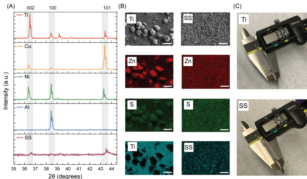
Fig. 4 (A) XRD spectra of electrodeposited Zn on different materials, at a fixed capacity of 0.5 \text{ mA h cm}^{-2} . (B) SEM and EDX mapping for Ti and SS. (Scale bar: 10 \text{ }\mu\text{m} .) (C) Thickness of Ti and SS coin cells is shown after 50 cycles.
