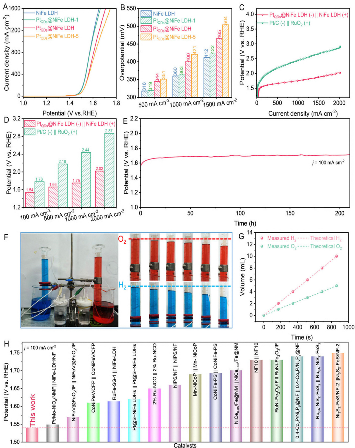
Fig. 11 OWS results; (A) LSV plots; (B) plot depicting comparison of overpotentials at different current densities; (C) potential vs. current density plots \text{Pt}_{\text{ODs}}@NiFe\ LDH\ (-) || NiFe\ LDH\ (+) and \text{Pt}/C\ (-) || RuO_2\ (+) ; (D) plot of potential (cell voltage) vs. current density (E) potential vs. time plot depicting stability in OWS process; (F) snapshots representing the OWS experimental set up and extent of gas collection at different instances; (G) plot depicting measured volume of H_2 or O_2 against theoretically produced H_2 or O_2 w.r.t. time; (H) potential comparison of \text{Pt}_{\text{ODs}}@NiFe\ LDH\ (-) || NiFe\ LDH\ (+) over other reported electrocatalysts (reproduced with permission from ref. 61 ©OAE publishing, Inc.; License: CC-BY 4.0).
