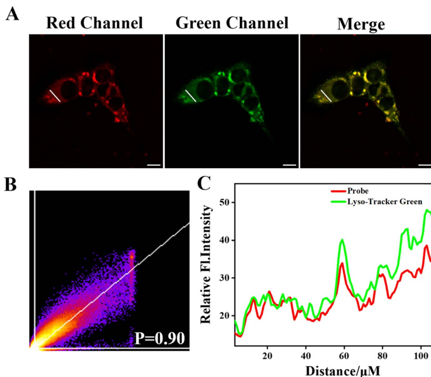
Fig. 8 (A) Co-localisation imaging of the probe LTP-H (10 μM) with LysoTracker™ Green (10 μM) in HepG-2 cells; red channel ( \lambda_{\text{ex}} = 590 nm, \lambda_{\text{em}} = 560 –700 nm); green channel ( \lambda_{\text{ex}} = 488 nm, \lambda_{\text{em}} = 500 –550 nm). (B) Correlation of the distribution of red-channel and green-channel fluorescence intensity. (C) Map showing the cellular ROI fluorescence intensity distribution. Scale bar: 10 μm.
