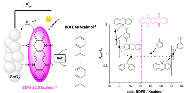
Fig. 13 QA based photoanode for oxidative C–H activation. The right figure shows the photoelectrochemical response (given by the ratio of the photocurrent in the presence and in the absence of the organic substrate) versus the BDFE of the C–H bond of the substrate. Reproduced from ref. 31 with permission from Wiley Inc., copyright 2023.
