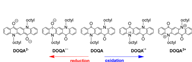
Scheme 2 Representation of oxidised and reduced forms of DOQA.
