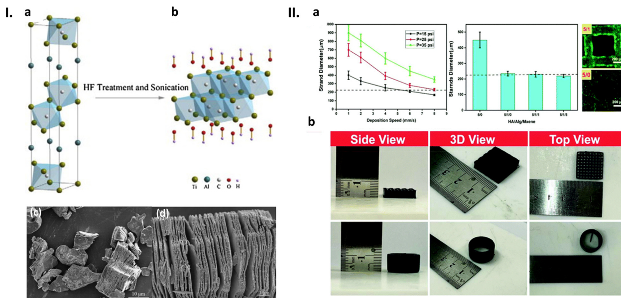
Fig. 32 (I) Preparation and structure of Ti_3C_2 MXene. (a) atomic structure of Ti_3AlC_2 ; (b) chemical structure of Ti_3C_2 , with OH termination ( Ti_3C_2 was made from Ti_3AlC_2 by HF etching and sonication); (c) and (d) SEM images of exfoliated Ti_3AlC_2 by 49% HF at 60 °C for 24 h. In (c), a low magnification is presented to show all grains are exfoliated, and in (d) a high magnification is used to show a fully exfoliated grain. Reproduced from ref. 529 with permission from Elsevier; copyright © 2015 Elsevier B.V. (II) Evaluation of the printability of MXene nanocomposite ink. (a) Finding the optimised operating parameters for extrusion-based 3D printing. (b) Pictures of 3D-printed structures fabricated using the MXene nanocomposite ink containing 1 \text{ mg mL}^{-1} Ti_3C_2 MXene nanosheets. Reproduced from ref. 256 with permission from The Royal Chemical Society; copyright © 2020.
