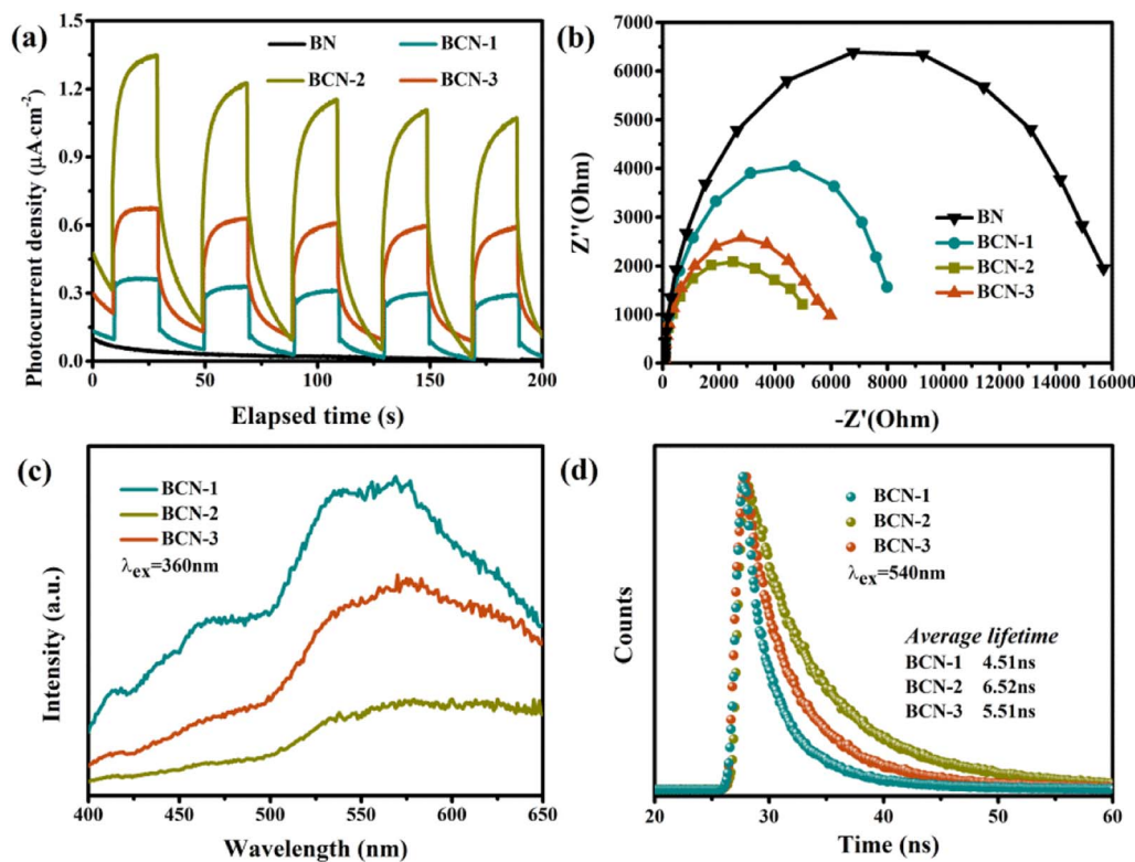
Fig. 5 (a) Transient photocurrent response curve of all samples, (b) electrochemical impedance spectroscopy (EIS) patterns of all BCN samples, (c) PL spectra of the BCN samples and (d) time-resolved photoluminescence (TRPL) spectra of all BCN samples.
