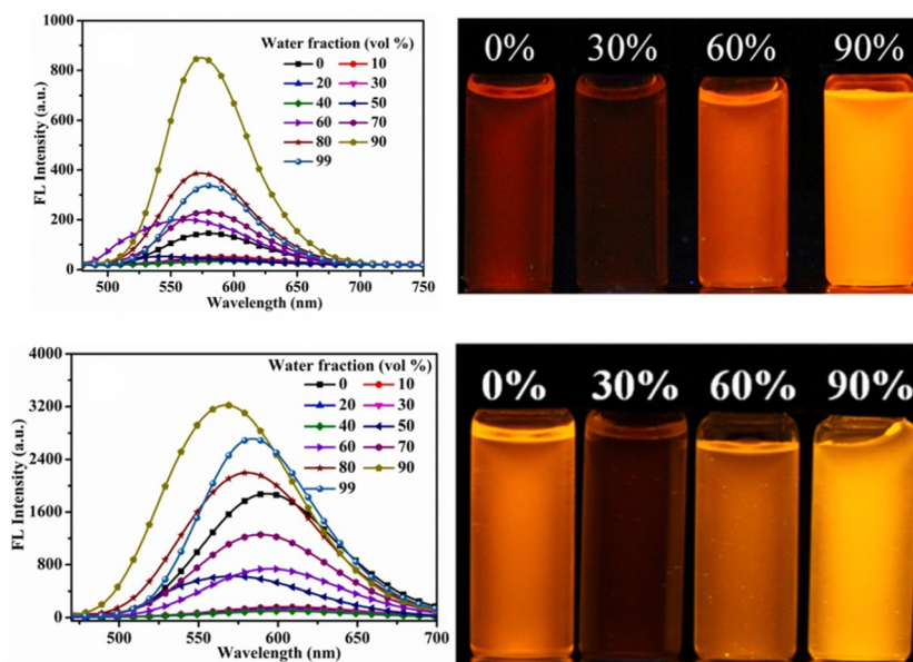
Fig. 5 Fluorescence spectra of compounds 4 and 6 with different fractions of water (left), and the corresponding images under 365-nm UV light (right). Reproduced with permission from ref. 75. Copyright 2021 Elsevier.
