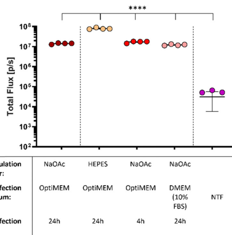
Fig. 5 Bioluminescent signals of in vitro saRNA-polyplex transfections with L-PEI 60 -ran-PPI 190 in HeLa cells. Cells (exposed to OptiMEM or full DMEM) were transfected with L-PEI 60 -ran-PPI 190 -based saRNA-polyplexes (N/P 5) containing 500 ng saRNA per well (24 well-plate). Polyplexes were formulated in HEPES (20 mM, pH 7.4; orange dots) or NaOAc (20 mM, pH 5.2). The graph shows data 24 hours after transfection, medium was not changed except for the pink dots, here OptiMEM medium was replaced by full DMEM/10% FBS 4 hours after transfection. Data was obtained with the IVIS Lumina III (Total Flux [p/s]). Each circle represents one well of the 24 well-plate ( N = 4 ), the line represents mean \pm SEM. *indicates significance of p \leq 0.05 , **indicates significance of p \leq 0.01 , ***indicates significance of p \leq 0.001 , ****indicates significance of p \leq 0.0001 . All conditions were compared to each other with one-way ANOVA, after log-transformation of the obtained data and testing for normality. Adjustment for multiple comparisons was performed using Tukey's multiple comparisons test. Abbreviations: NTF = non-transfected cells.
