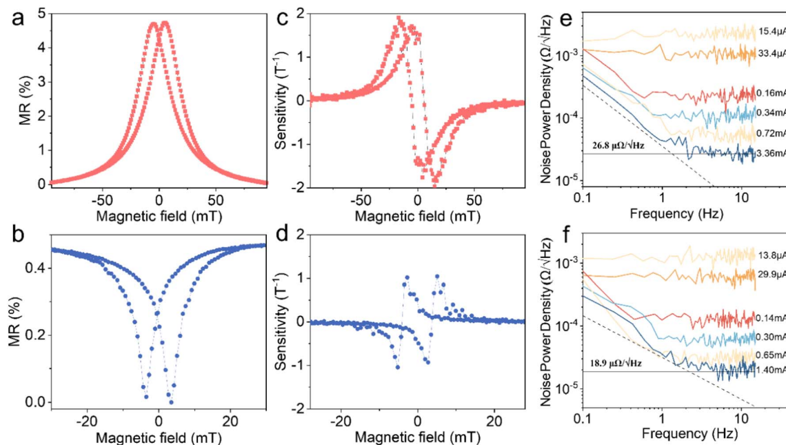
Fig. 2 Magneto-electric performance of printed magneto-resistive sensors. (a) MR, (c) sensitivity and (e) noise of the printed sensor with [\text{Co}/\text{Cu}]_{50} GMR microflakes as functional fillers. (b) MR, (d) sensitivity and (f) noise of the printed sensor with \text{Ni}_{97}\text{Co}_3 AMR microparticles as functional fillers. All measurements are performed at room temperature.
