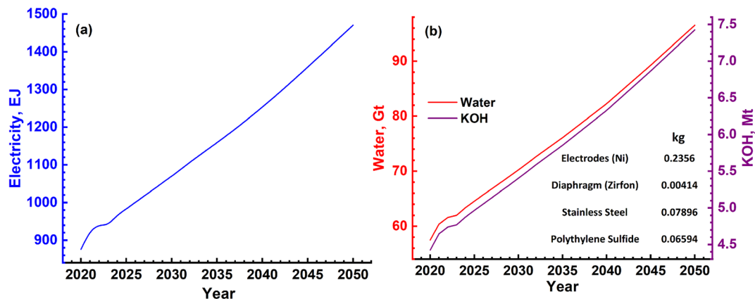
Fig. 12 (a) Electrolysis process requires a significant amount of electrical energy annually for splitting water. This will increase to \sim 1500 EJ by the year 2050 and become highly critical. (b) The corresponding annual requirement for water and the electrolyte KOH. The water requirement is of the order of several Gt each year. The magnitudes of other electrolytic cell materials such as electrodes, separators and sealants required to produce 1 kg of H_2 gas are given in the inset of (b). It can be seen that the supply of these materials can become critical with the increase in H_2 production.
