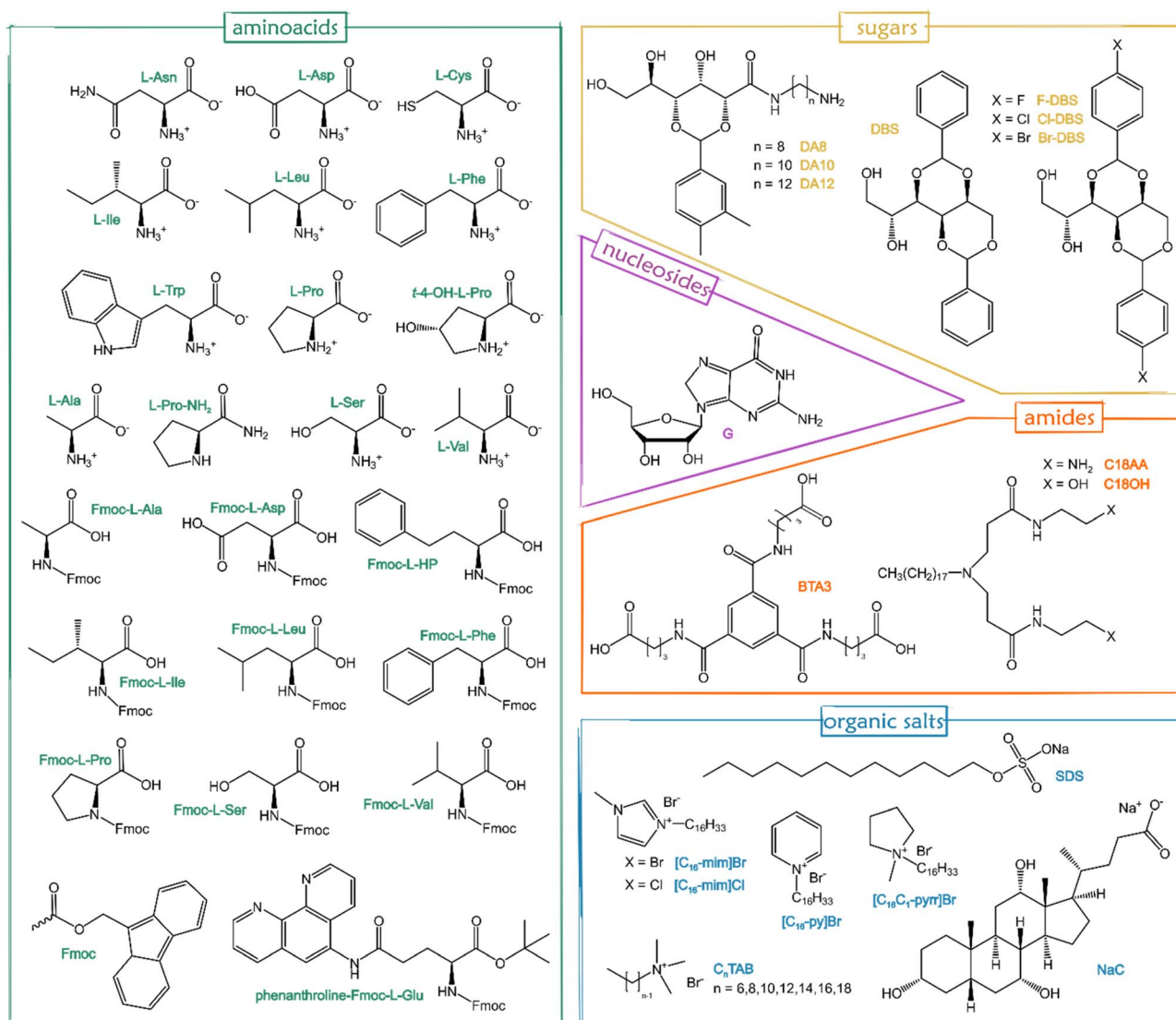
Fig. 6 Low molecular weight gelators (LMWGs) discussed in this review. Abbreviations: BGA-10, 1,10-diguconaminodecane; BGA-12, 1,12-diguconaminododecane; BTA3, N,N,N' -tri hexanoic acid benzene-1,3,5-tricarboxamide; C18AA, long alkylaminoamide derivative with two terminal primary amine moieties; C18OH, long alkylaminoamide derivative with two terminal hydroxyl moieties; C n TAB, alkyl trimethyl ammonium bromide; [C 16 -mim]Br, 1-hexadecyl-3-methylimidazolium bromide; [C 16 -py]Br, N -hexadecylpyridinium bromide; [C 16 -py]Cl, N -hexadecylpyridinium chloride; [C 16 C 1 -pyrr]Br, N -hexadecyl- N -methylpyrrolidinium bromide; Dan, D-gluconic acetal; DBS, 1,3,2,4-dibenzylidene-β-D-sorbitol; Fmoc, 9-fluorenylmethoxycarbonyl protecting group; G, guanosine; L-Ala, L-alanine; L-Asn, L-asparagine; L-Asp, L-aspartic acid; L-Cys, L-cysteine; L-HP, L-homophenylalanine; L-Ile, L-isoleucine; L-Leu, L-leucine; L-Phe, L-phenylalanine; L-Pro, L-proline; L-Pro-NH 2 , L-prolinamide; L-Ser, L-serine; L-Trp, L-tryptophan; L-Val, L-valine; phenanthroline-Fmoc-L-Glu, phenanthroline-derivative of N -α-Fmoc-L-glutamic acid α- tert -butyl ester; NaC, sodium cholate; SDS, sodium dodecyl sulfate; t -4-OH-L-Pro, trans -4-hydroxy-L-proline.
