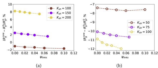
Fig. 5 Signed difference between the gyration radius of the core R_g^{\text{core}} of core-shell nanogels and the gyration radius of the original nanogel R_g^0 in a good solvent as a function of the fraction of cross-linked monomers on the shell \psi_{\text{links}} . (a) M_{\text{sh}} = 10 and (b) M_{\text{sh}} = 20 monomers each. Brown colour corresponds to nanogels with N^{\text{sh}} = 1000 monomers in the shell, purple – N^{\text{sh}} = 1500 , and yellow one for N^{\text{sh}} = 2000 .
