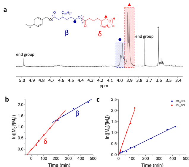
Fig. 3 (a) 1 H NMR spectrum (CDCl 3 , 400 MHz) of \beta and \delta -C 18 PCL. * = MeOH. (b) Semi-logarithmic kinetic plot for the ROP of \beta/\delta -C 18 CL isomers. (c) Resolved semi-logarithmic kinetic plot for the ROP of \beta/\delta -C 18 CL isomers. [M]_0 = 0.5 M (calculated by NMR spectroscopy based on a starting ratio of \beta isomer : \delta isomer = 1 : 1).
