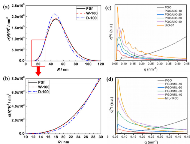
Fig. 5 (a and b) Pore volume distributions of PSf, PDMS/PSf (wet) (W-100) and PDMS/PSf (dry) (D-100) membranes. Reproduced with authorisation from ref. 58 and copyright 2019 by Elsevier. (c and d) SAXS patterns of MMMs containing UiO-67 or MIL-140C. Reproduced with authorisation from ref. 60 and copyright 2022 by Elsevier.
