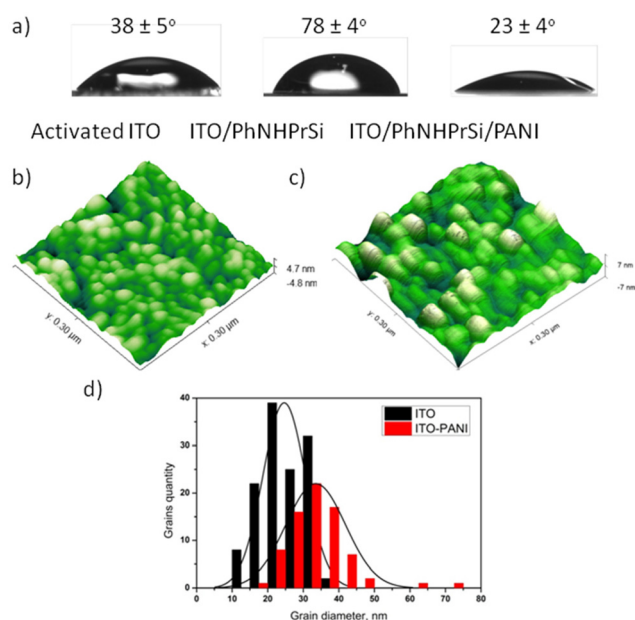
Fig. 1 Properties of the ITO/PhNHPrSi/PANI surface: (a) the averaged water contact angles of the bare ITO, ITO/PhNHPrSi, and ITO/PhNHPrSi/PANI surfaces; (b) AFM image of the bare ITO and (c) the ITO/PhNHPrSi/PANI surfaces; (d) the statistical distributions of grain diameters (the histograms are mean distributions of the grains diameters) on the surfaces.
