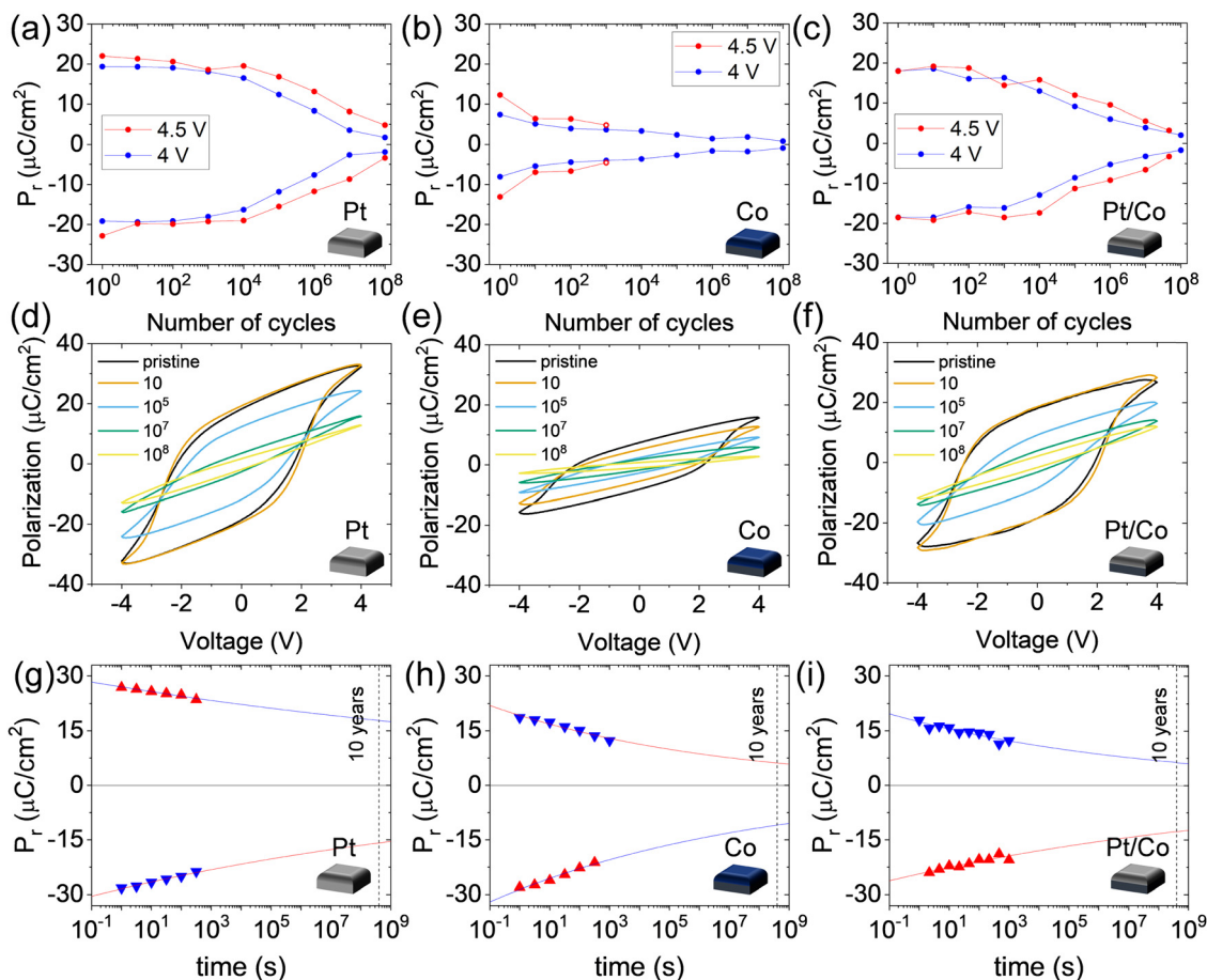
Fig. 3 (a)-(c) Endurance, measured with bipolar rectangular pulses of frequency 100 \text{ kHz} and amplitude of indicated voltage using Pt, Co and Pt/Co top electrodes, respectively. (d)-(f) P - V loops measured after the indicated number of cycles using Pt, Co and Pt/Co top electrodes, respectively. (g)-(i) Retention of the samples using Pt, Co and Pt/Co top electrodes, respectively.
