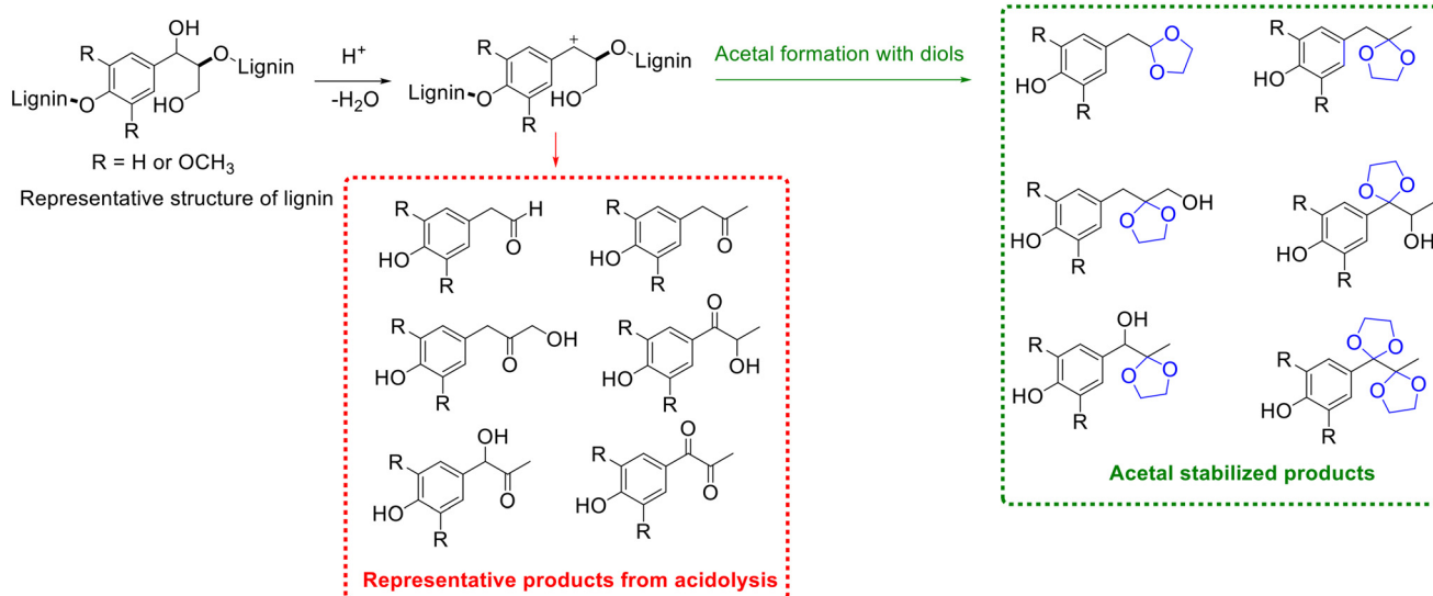
Scheme 11 Representative products or acetal stabilized products from lignin \beta -O-4 linkage acidolysis.
