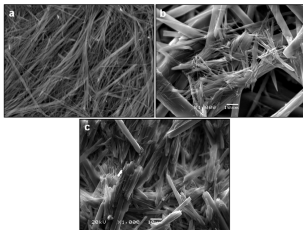
Fig. 5 SEM images of (a) Phe (303 mM), (b) Phe/NH 2 -Phe (1 : 2) and (c) NH 2 -Phe (606 mM) dried hydrogels. The hair-like fibres of Phe had an average width of 1.1 \mu\text{m} (ranging between 0.4 and 1.7 \mu\text{m} ), whereas the average width of the needle-like fibres of NH 2 -Phe was 25.3 \mu\text{m} (ranging between 2.6 and 47.9 \mu\text{m} ).
